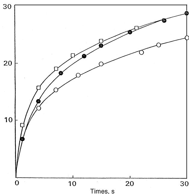
Figure 9. Consumption of ethene (initial pressure of 1.67 kPa) with time during the oligomerization at room temperature in the presence of the samples 0.9NAS-Ex (○), 3.5NAS (□) and the sample obtained by additional loading of Ni(II) (see the text) over the 0.9NAS sample (●). The catalysts are thermoactivated at 773 K.
