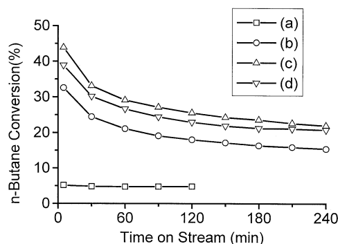
Figure 7. Catalytic activity of catalysts calcined at 680 °C at constant \text{ZrO}_2 content 50 wt% with various Ga contents. (a) 0.0 wt%; (b) 0.57 wt%; (c) 1.7 wt%; (d) 2.84 wt%.
