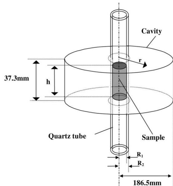
Figure 1. Schematic of the resonant cavity with the sample and its holder.
