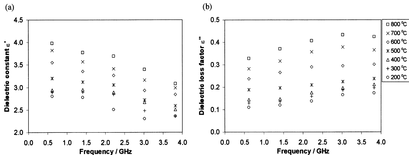
Figure 8. Dielectric properties of mechanically mixed catalyst MoS 2 + \gamma -Al 2 O 3 versus microwave frequency at different temperatures.
