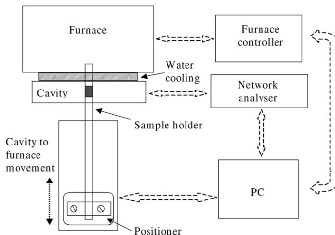
Figure 2. The experimental system for the dielectric property measurements.
