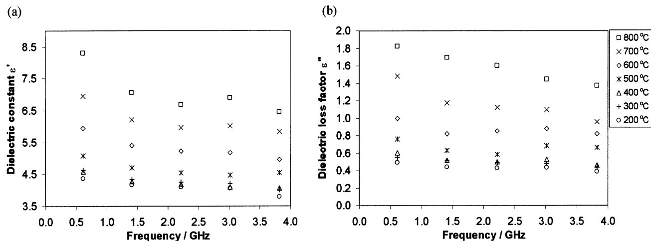
Figure 9. Dielectric properties of impregnated catalyst MoS 2 / \gamma -Al 2 O 3 versus microwave frequency at different temperatures.
