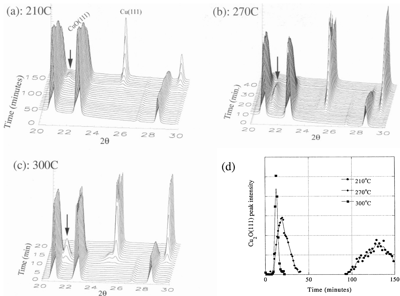
Figure 3. Time-resolved XRD data for the reduction of CuO under a 5% \text{H}_2 /95% He mixture (flow rate \sim 1 \text{ cm}^3/\text{min} ) at three different temperatures: (a) 210, (b) 270 and (c) 300 °C. The arrows indicate the main diffraction line for \text{Cu}_2\text{O} . (d) Intensity of the main diffraction line for \text{Cu}_2\text{O} in each case.
