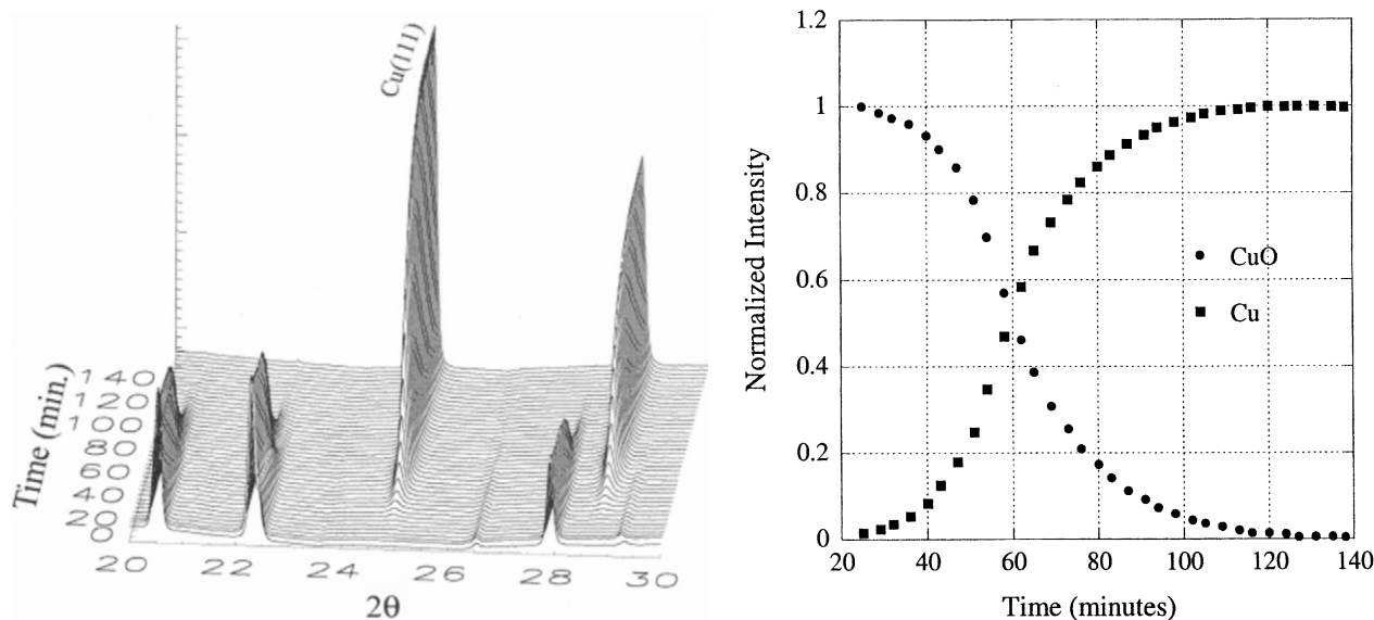
Figure 2. Left: time-resolved XRD data for the reduction of CuO under a 5% H 2 /95% He mixture (flow rate \sim 20 cm 3 /min) at 200 °C. Right: amounts of CuO and Cu present as a function of time.
