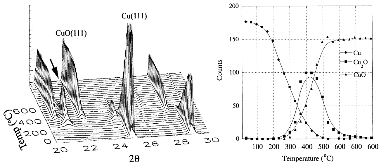
Figure 8. Time-resolved XRD data for the oxidation of Cu under a 5% O 2 /95% He mixture (flow rate \sim 20 cm 3 /min) at 25–600 °C and constant 600 °C (30 min). The arrow indicates the main diffraction line for Cu 2 O. In the right-hand-side graph is shown the variation of the main diffraction lines for Cu, Cu 2 O and CuO as a function of temperature.
