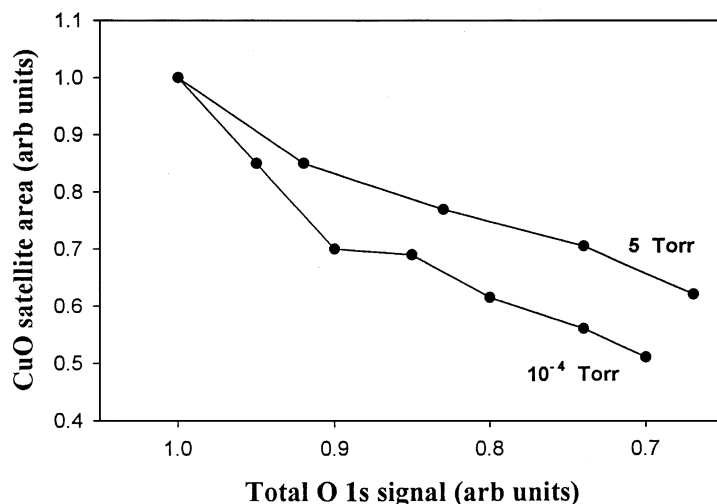
Figure 6. Relationships between the decreases in the CuO Cu 2p satellite area and total O 1s signal for the reduction of CuO under 10^{-4} and 5 torr of H_2 .
