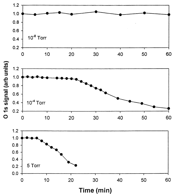
Figure 4. Variation of the O 1s signal as a function of time for the reduction of CuO films at 200 °C under different pressures of H 2 .
