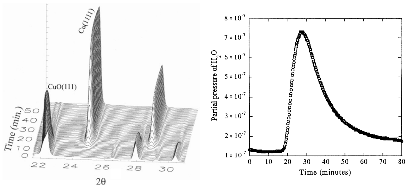
Figure 1. Left: time-resolved XRD data for the reduction of CuO under a 5% H 2 /95% He mixture (flow rate \sim 20 cm 3 /min) at 240 °C. Right: evolution of water during the reduction process.
