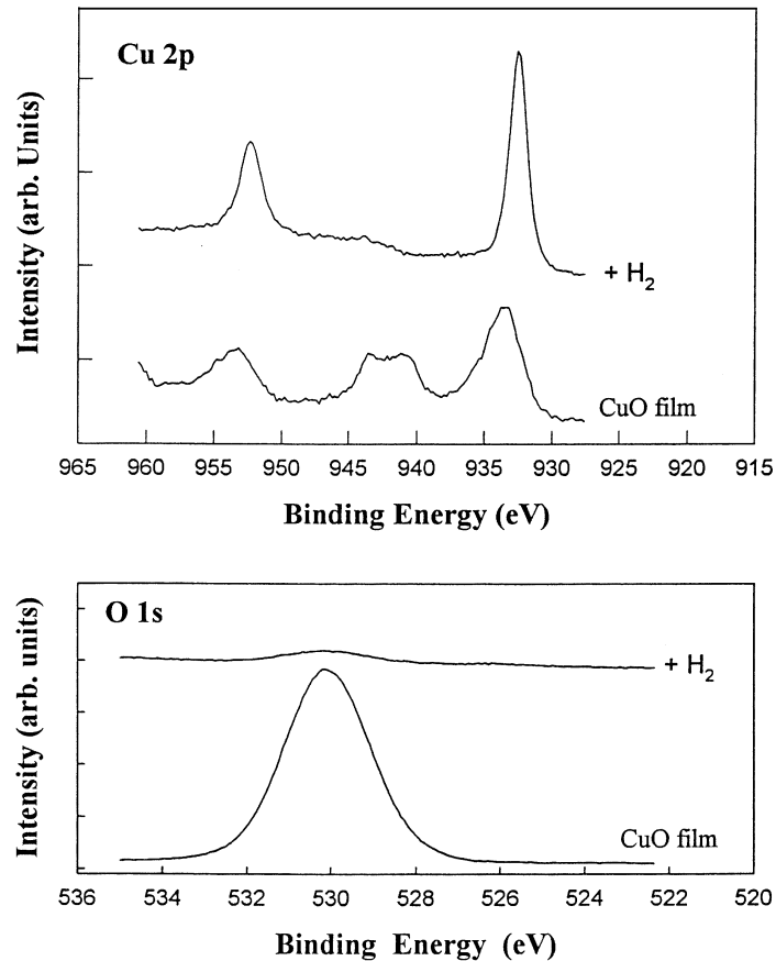
Figure 5. Cu 2p (top panel) and O 1s (bottom panel) XPS spectra taken before and after partial reduction of a CuO film with H 2 at 200 °C.
