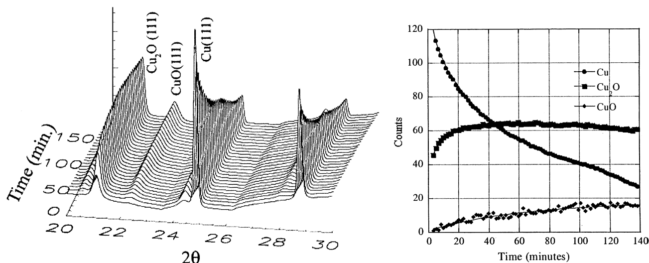
Figure 7. Time-resolved XRD data for the oxidation of Cu under a 5% O_2 /95% He mixture (flow rate \sim 20 \text{ cm}^3/\text{min} ) at 300^\circ\text{C} . In the right-hand-side graph is shown the variation of the main diffraction lines for Cu, Cu_2O and CuO as a function of time.
