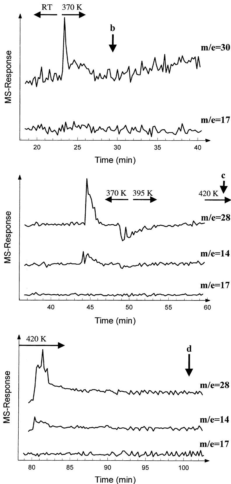
Figure 4. Mass spectrometer signal of NO ( m/z = 30 ) and N_2 ( m/z = 28.14 ) normalized on the ion current of ammonia ( m/z = 15 ) are plotted as a function of time. The masses m/z = 14 , 15 and 17 represent fragments of ammonia. The straight line of m/z = 17 after normalization demonstrates the successful removal of artifacts. Since the peaks of m/z = 14 at 44 min (370 K) and 81 min (420 K) coincide with peaks in m/z = 28 , it can be concluded that the signal is due to the formation of nitrogen. The temperature of the catalyst is indicated. The time scale is given relative to the detection moment of NEXAFS spectrum (a) in figure 3. The detection moment of NEXAFS spectra b, c and d (figure 3) is indicated by arrows in the plot.
