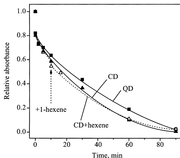
Figure 6. Conversion of CD and QD on a 5 wt% Pd/TiO 2 catalyst in the presence of hydrogen and, alternatively, also 1-hexene as a model reactant. The hydrogenation reactions are followed by UV-vis spectroscopy. Conditions: 1 bar and room temperature, 40 mg 5 wt% Pd/TiO 2 , 20 ml 2-propanol, 3.4 \mu mol modifier. Addition of 2 ml 1-hexene after 10 min hydrogenation of CD (open symbols, dashed line).
