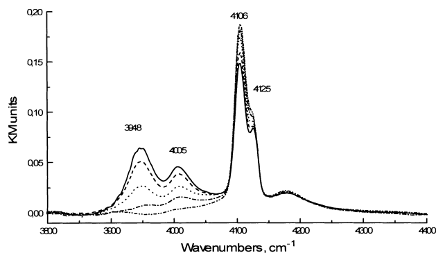
Figure 5. DRIFT spectra of hydrogen adsorbed at 77 K by HZSM-5(25) with 1% of modifying Zn ions pretreated in vacuum at 300 °C (.....), 400 °C (-----), 500 °C (.....), 600 °C (-----) or 650 °C (——). DRIFT measurements at 77 K.
