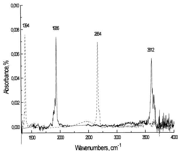
Figure 8. Transmittance IR spectra of \text{H}_2 (solid line) and \text{D}_2 (dashed line) adsorbed on HZSM-5 with \text{Si}/\text{Al} = 41 modified with 4% of \text{Zn}^{+2} ions at room temperature and equilibrium pressure of 50 Torr.
