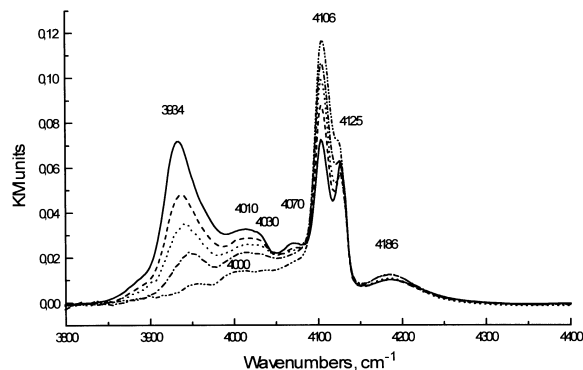
Figure 7. DRIFT spectra of hydrogen adsorbed at 77 K by HZSM-5(80) with 1% of modifying Zn ions pretreated in vacuum at 300 °C (.....), 400 °C (-----), 500 °C (.....), 600 °C (-----) or 650 °C (——). DRIFT measurements at 77 K.
