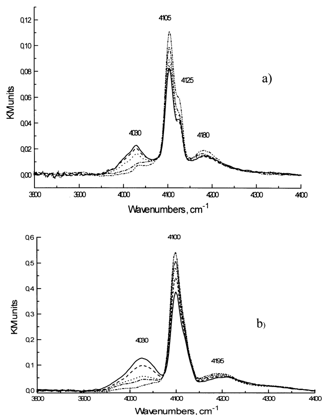
Figure 1. DRIFT spectra of H 2 adsorbed at 77 K by HZSM-5(41) (a) and HMOR(5) (b) pretreated in vacuum at 300 °C (·····), 400 °C (— · — · —), 500 °C (— · — · —), 600 °C (— · — · —) or 650 °C (——). DRIFT measurements at 77 K.
