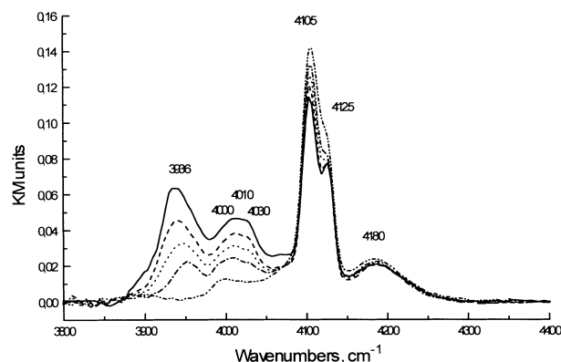
Figure 6. DRIFT spectra of hydrogen adsorbed at 77 K by HZSM-5(41) with 1% of modifying Zn 2+ ions pretreated in vacuum at 300 °C (.....), 400 °C (-----), 500 °C (.....), 600 °C (-----) or 650 °C (——). DRIFT measurements at 77 K.
