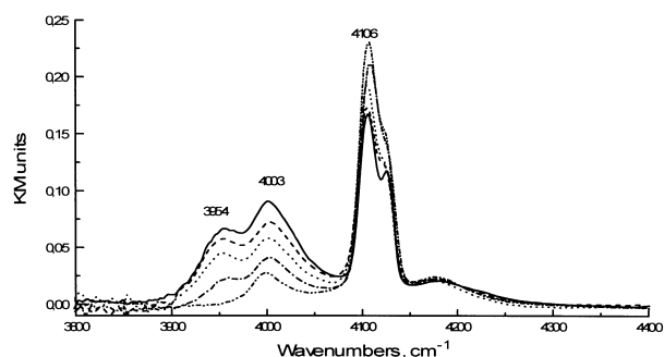
Figure 4. DRIFT spectra of hydrogen adsorbed at 77 K by HZSM-5(15) with 1% of modifying Zn ions pretreated in vacuum at 300 °C (.....), 400 °C (-----), 500 °C (.....), 600 °C (-----) or 650 °C (——). DRIFT measurements at 77 K.
