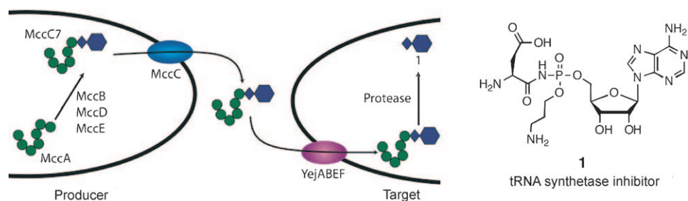
Figure 13. Left: Transport and antibiotic mechanism of action of MccC7. Right: Structure of the toxic aspartyl-AMP analogue. The N–P bond provides hydrolytic stability.
