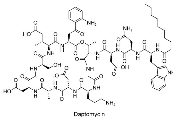
Figure 2. Examples of nonribosomally synthesized antibiotic peptides. Cross-linking of the vancomycin heptapeptide provides a dome-shaped architecture. Tailoring of the ACV tripeptide creates the rigidified \beta -lactam moiety of isopenicillin N. Daptomycin undergoes macrocyclization during release from its NRPS.
