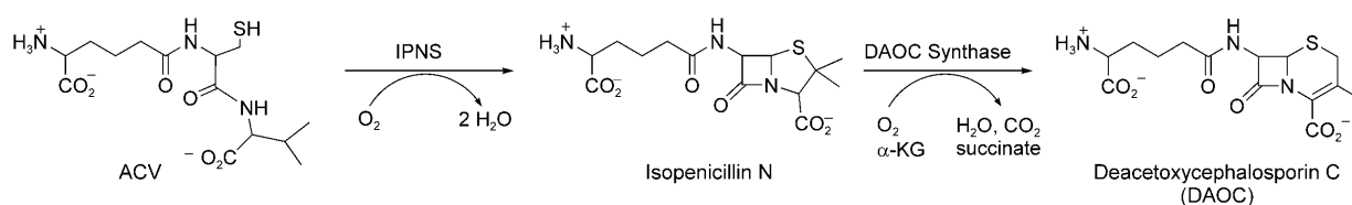
Figure 20. Conversion of ACV to isopenicillin N and deacetoxycephalosporin C (DAOC) by the successive action of two nonheme iron oxygenases IPNS and DAOC synthase.
