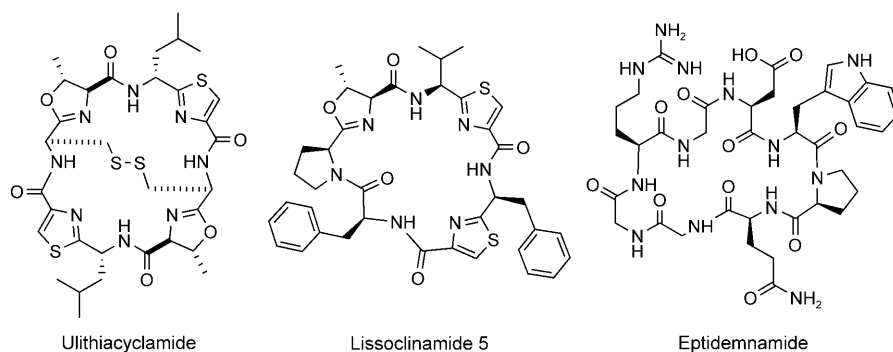
Figure 11. Additional cyanobactins generated by patE variants.
