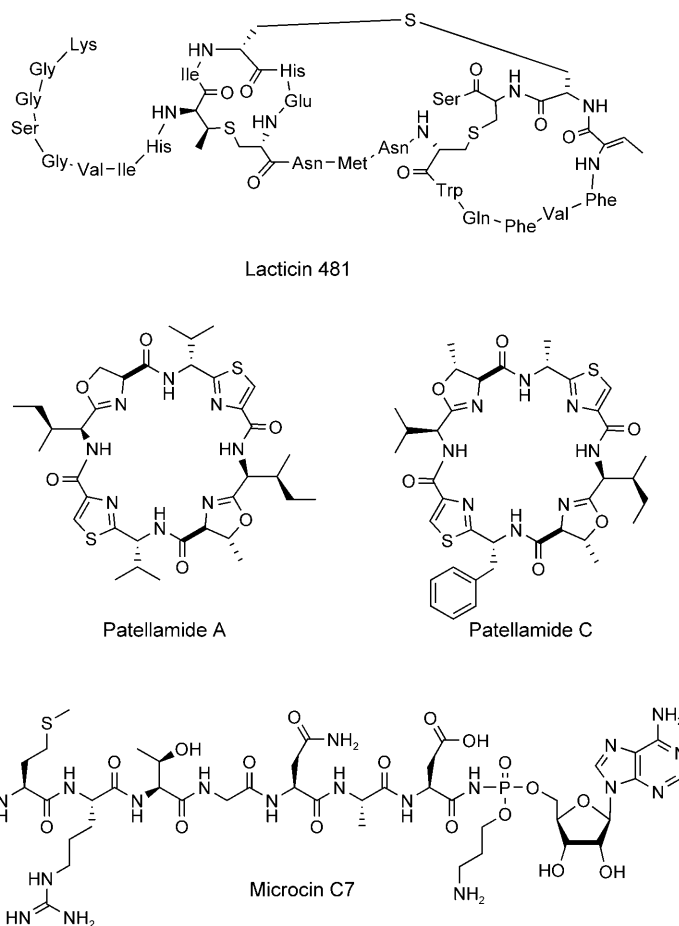
Figure 1. Examples of ribosomally synthesized peptides that undergo post-translational modification. Lactacin 481 contains two lanthionines, one methyllanthionine, and one 2,3-didehydrobutyrine, all of which result from post-translational tailoring. Patellamide A and C are octapeptides that become macro- and heterocyclized during maturation. Microcin C7 exhibits an unusual C-terminal appendage that is comprised of an aminopropyl-modified AMP moiety that is linked to the peptide by a N–P bond.
