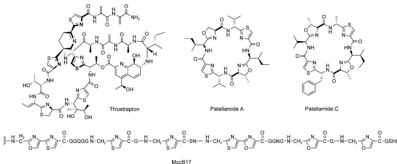
Figure 7. Examples of antibiotic peptides that contain five-membered heterocycles derived from cysteine or serine/threonine. The first twelve residues of MccB17 (VGIGGGGGGGGG) are omitted.
