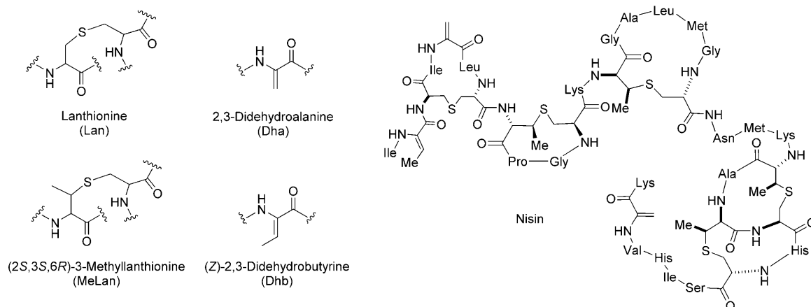
Figure 5. Structures of lanthionine (Lan), (2S,3S,6R)-3-methylanthionine (MeLan), 2,3-didehydroalanine (Dha), (Z)-2,3-didehydrobutyryne (Dhb), and nisin.
