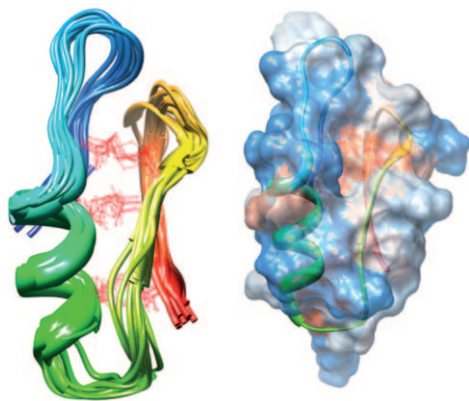
Figure 3. NMR spectroscopic solution-phase structures of plectasin (PDB ID: 1ZFU). The disulfide linkages are shown in red. The image is colored from blue to red going from the N to C terminus.
