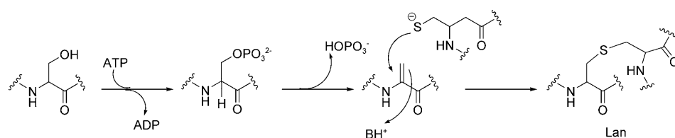
Figure 6. Formation of lanthionine. Dehydration of a serine residue in the peptide backbone affords Dha. A cysteine thiolate captures the eneamino acid side chain of Dha to form the thioether.
