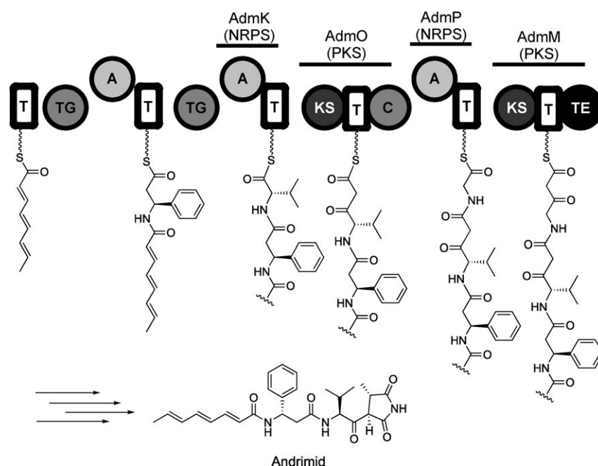
Figure 24. Depiction of the andrimid assembly line illustrating N-acylation of \beta -Phe and formation of the methylsuccinimide precursor chain. Abbreviations: TG = transglutaminase-like enzyme; KS = ketosynthase.
