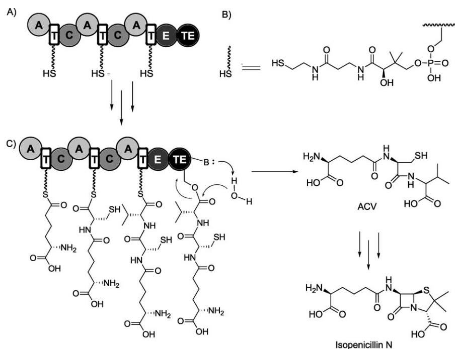
Figure 19. Chain growth and release of ACV on the ACV synthetase assembly line. A) Post-translationally primed ACV synthetase. B) Structure of the phosphopantetheinyl arm. C) ACV Chain elongation and release. Further enzymatic modification of ACV affords isopenicillin N. "E" stands for epimerase domain.
