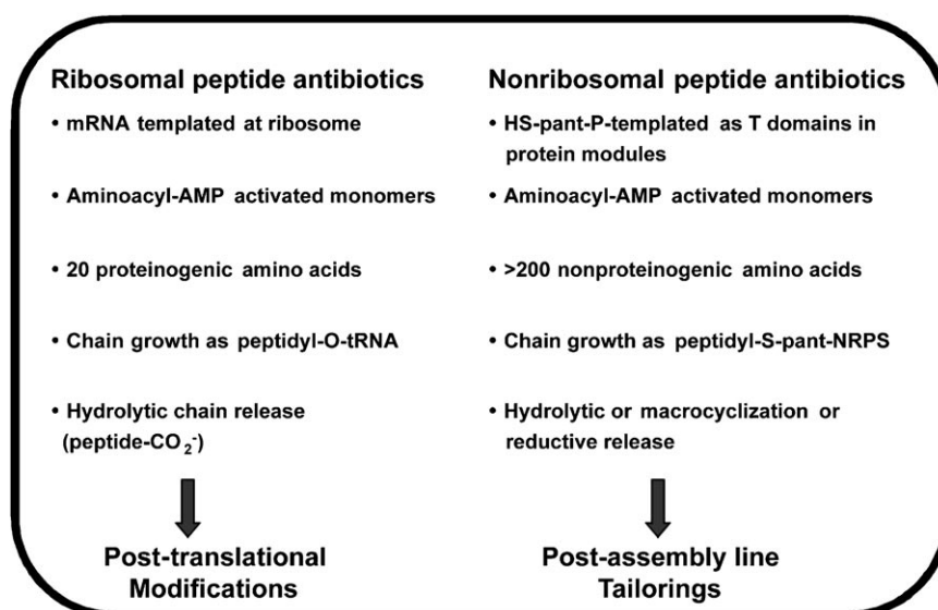
Figure 17. Comparison of ribosomal and nonribosomal peptide antibiotic synthesis. "Pant" stands for "phosphopantetheinyl."
