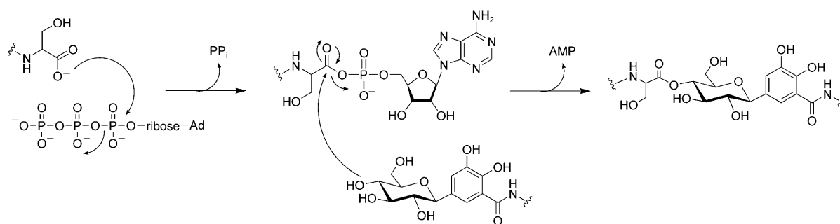
Figure 16. Mechanism of C-terminal activation and glycosyl ester formation by MceIJ. Only the C-terminal serine residue of MccE492 and a truncated depiction of MGE are shown for clarity.
