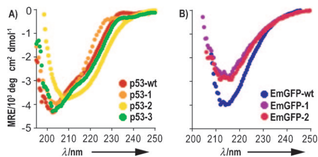
Figure 2. Circular dichroism (CD) spectra for p53 and EmGFP bipartite display variants. A) Wavelength-dependent CD spectra of 8.1 \mu\text{M} p53-wt (wild type), 8.1 \mu\text{M} p53-1, 8.1 \mu\text{M} p53-2, and 8.1 \mu\text{M} p53-3. B) Wavelength-dependent CD spectra of 25 \mu\text{M} EmGFP-wt, 25 \mu\text{M} EmGFP-1 and 25 \mu\text{M} EmGFP-2. CD data were acquired at 25 °C in 100 mM Tris-HCl, 75 mM NaCl, and 3.5 mM TCEP (pH 7.8) in the absence of competing dithiols (EDT). MRE = mean residue ellipticities.
