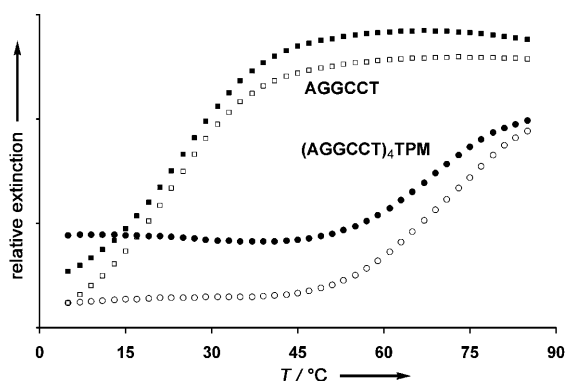
Figure 4. UV-melting (heating curves: open symbols, cooling curves: filled symbols) of a hybrid with four self-complementary hexanucleotide DNA arms (4 \mu\text{M} ) and the corresponding linear control (16 \mu\text{M} ) in 10 mM TEAA buffer, 150 mM NaCl, pH 7. Raw data of melting curves can be found in the Supporting Information.
