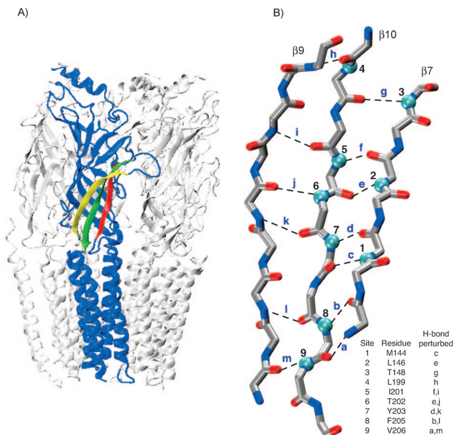
Figure 1. Two views of the nAChR. A) Overall layout of the receptor. One of the five subunits is shown in blue, with \beta 7 , \beta 9 , and \beta 10 highlighted in red, yellow, and green, respectively. B) The hydrogen bonding network of the outer \beta sheet of the nAChR. Turquoise balls indicate the positions at which the backbone NH was mutated to an oxygen atom. The black dashed lines indicate hydrogen bonds that are completely removed or attenuated as a result of mutation. The image is based on the cryoelectron micrograph of the full Torpedo receptor (PDB ID: 2BG9). [18]
