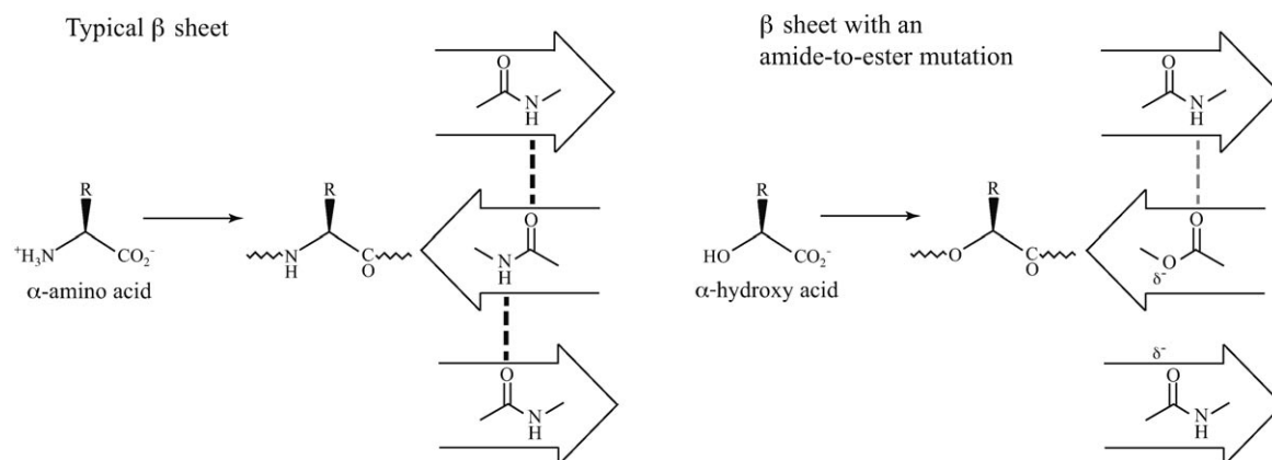
Scheme 1. Schematic representation of the backbone amide versus the backbone ester bond in the context of a \beta sheet.
