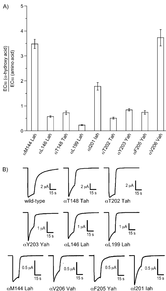
Figure 2. Characteristics of nAChR with backbone mutations in \beta strands 7 and 10. A) EC_{50} shifts for backbone mutations made at nine positions in \beta 7 and \beta 10 . Modest effects on receptor function are observed in all cases. B) Current traces for backbone mutations made at nine positions in \beta 7 and \beta 10 .
