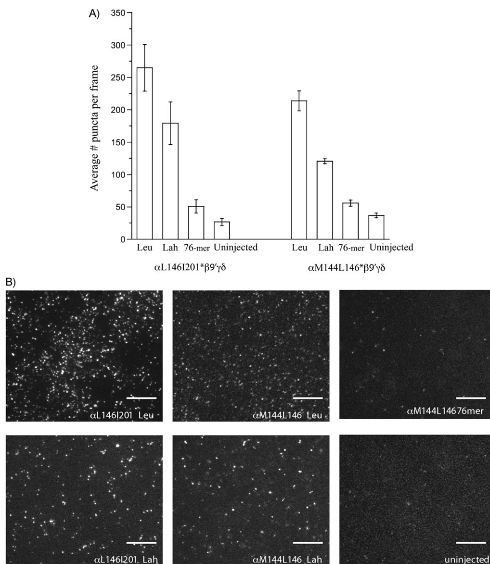
Figure 3. Analysis of dysfunctional nAChRs containing two amide-to-ester mutations by TIRF microscopy. A) Puncta density for receptors labeled with Leu refers to recovery of the wild-type peptide backbone by nonsense suppression; Lah refers to incorporation of leucine \alpha -hydroxy; 76-mer indicates the negative control experiment (co-injection of mRNA with a tRNA molecule that has not been charged with an amino or hydroxy acid). The puncta density for both Leu and Lah are significantly higher than that of either the 76-mer or uninjected oocyte controls (t-test values for Lah versus 76-mer are: P = 0.0009 (L146I120); P < 0.0001 (L146M144); for Lah versus uninjected: P = 0.0003 (L146I120); P < 0.0001 (L146M144). Data are compiled from \geq 6 non-overlapping images from \geq 2 oocytes. B) Representative TIRF images corresponding to the data in (A); scale bar: 6 \mu\text{m} .
