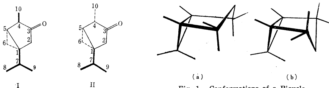
Fig. 1. Conformations of a Bicyclo-[3.1.0]hexane Ring
