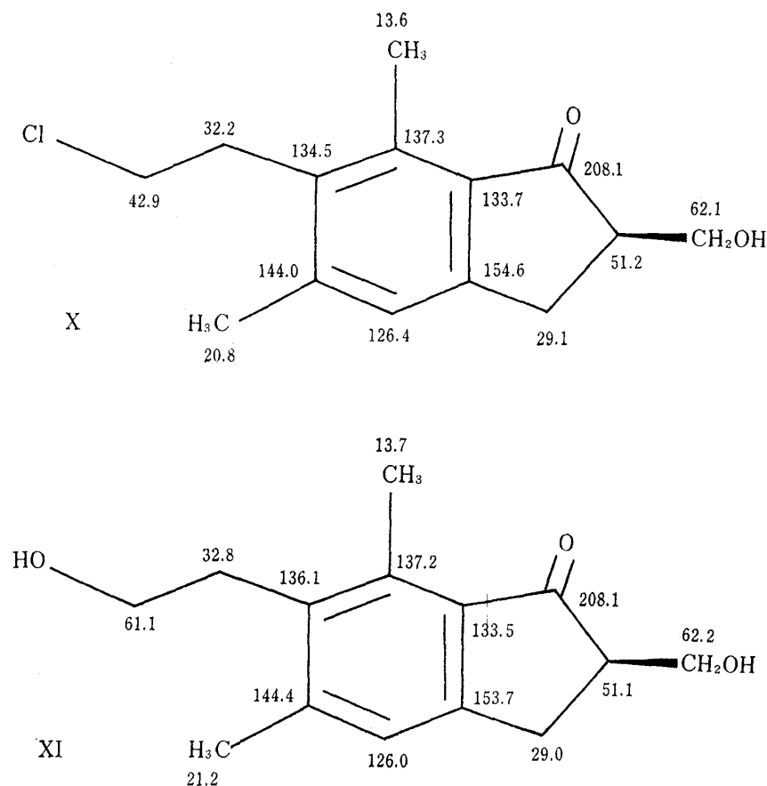
Fig. 2. ^{13}\text{C} Chemical Shifts in Pyridine- d_6
