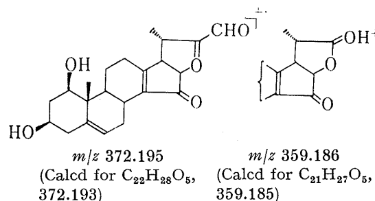
Fig. 7. Probable Structures of Fragments ( m/z 372 and 359) Seen in the Mass Spectrum of 21-Deoxytrillenogenin (XXIII)
