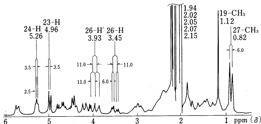
Fig. 1. PMR Spectrum of Epitritillenogenin Acetate (XIII)
