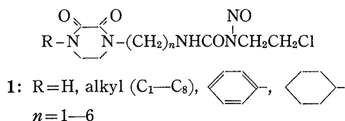
Chart 1. Chemical Structure of 1-(2-Chloroethyl)-3-(4-substituted-2,3-dioxo-1-piperazinyl)alkyl-1-nitroso-urea
