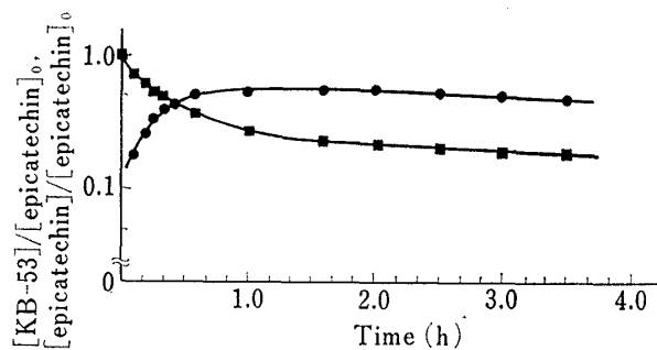
Fig. 7. Disappearance of Epicatechin and Appearance of KB-53 at pH 10.7 and 40°C
