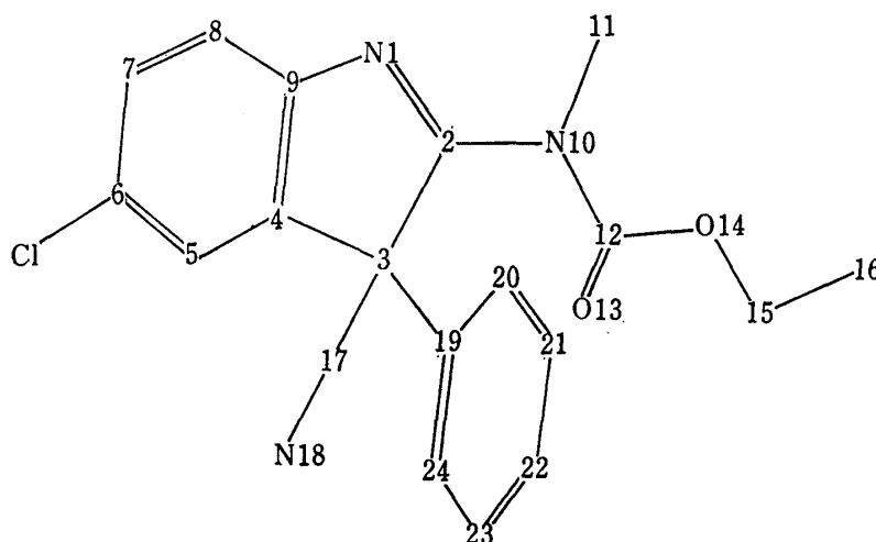
Fig. 1. Atomic Numbering of Compound 4
