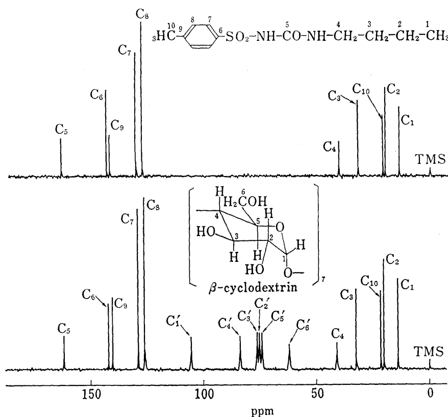
Fig. 1. ^{13}\text{C} NMR Spectra of Tolbutamide (Top) and Tolbutamide/ \beta -Cyclodextrin (Bottom) in Solution
