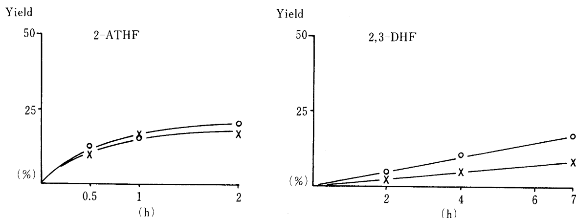
Fig. 4. Isotopic Effect
