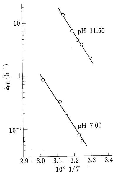
Fig. 7. Arrhenius Plots of the Apparent First-Order Rate Constants, k_{\text{pH}} , for Cefatrizine Degradation at pH 7.00 and 11.50, and an Ionic Strength of 0.5.
