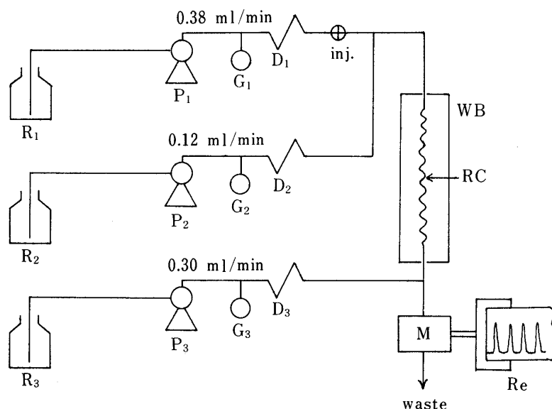
Fig. 1. Schematic Diagram of the FIA System
