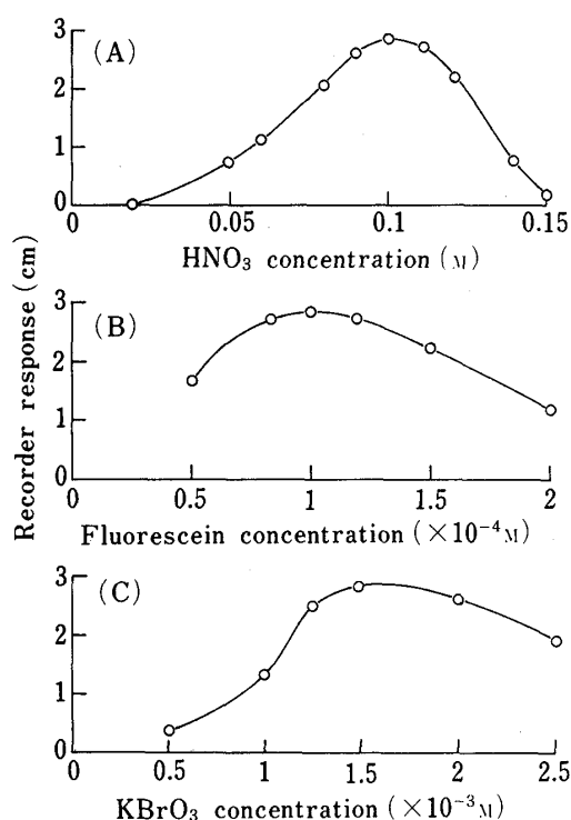
Fig. 2. Effects of Concentrations of HNO 3 , Fluorescein and KBrO 3 on the Peak Height
