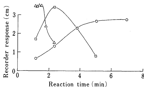
Fig. 3. Effect of Reaction Time at Various Temperatures on the Peak Height
