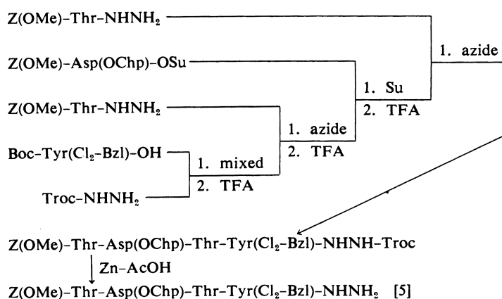
Fig. 3. Synthetic Scheme for the Protected Tetrapeptide Hydrazide (Positions 7—10)
