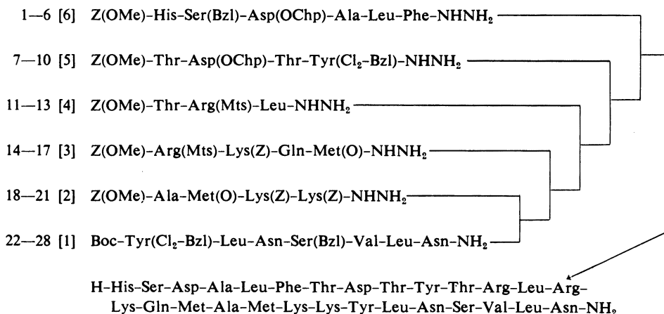
Fig. 1. Synthetic Route to Guinea Pig VIP (gVIP)
