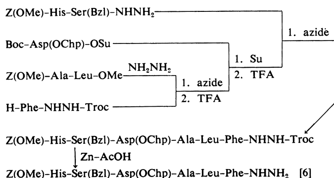
Fig. 4. Synthetic Scheme for the Protected N-Terminal Hexapeptide Hydrazide (Positions 1—6)
