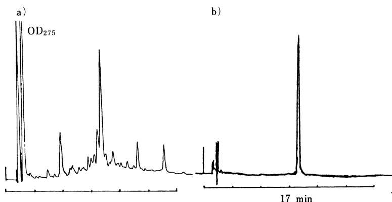
Fig. 6. HPLC (Cosmosil 5C18 Column) of Synthetic gVIP
