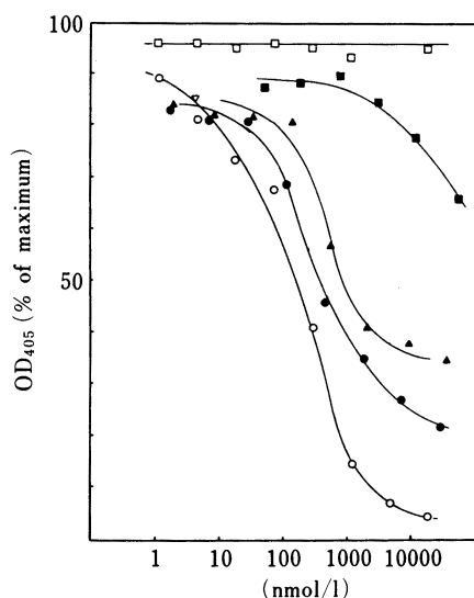
Fig. 5. Immunological Properties of Synthetic gVIP
