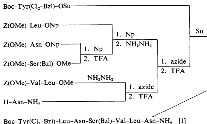
Fig. 2. Synthetic Scheme for the Protected C-Terminal Heptapeptide Amide (Positions 22—28)
