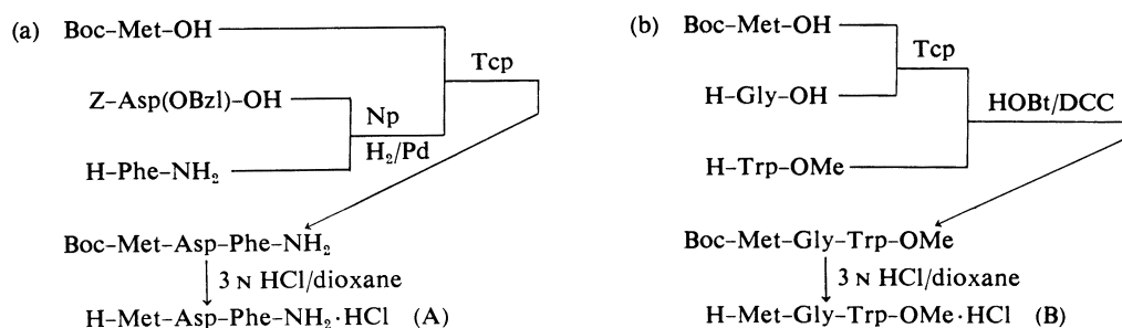
Fig. 2. Synthetic Schemes for the C-Terminal (A) and the Middle (B) Fragments
