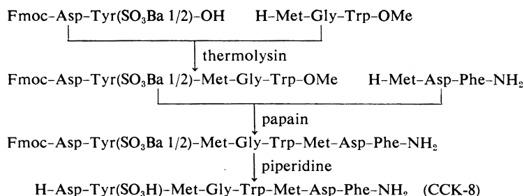
Fig. 1. Synthetic Scheme for CCK-8
