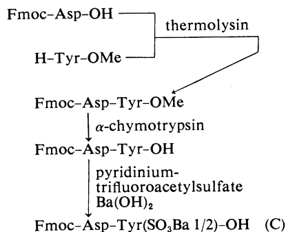
Fig. 3. Synthetic Scheme for the N-Terminal Fragment (C)
