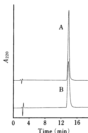
Fig. 4. HPLC Comparison of Enzymatically Synthesized CCK-8 (A) and Chemically Synthesized CCK-8 (B)
