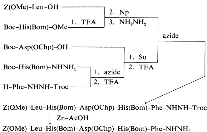
Fig. 3. Synthetic Scheme for the Protected Pentapeptide Hydrazide [2] (Positions 25–29)
