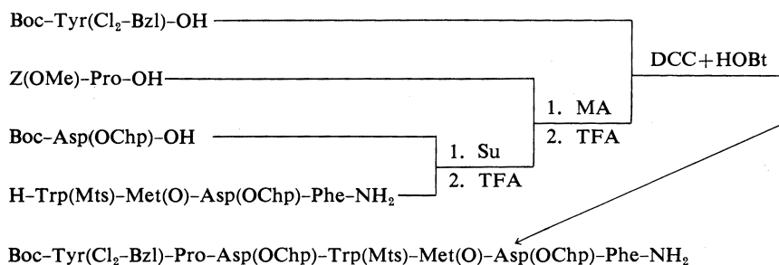
Fig. 2. Synthetic Scheme for the Protected Heptapeptide Amide [1] (Positions 30—36)
