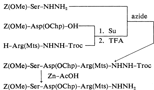
Fig. 6. Synthetic Scheme for the Protected Tripeptide Hydrazide [5] (Positions 10—12)
