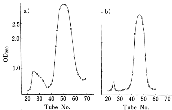
Fig. 9. Gel-Filtration of Protected Antral Peptide a) Eluted with DMF. b) Eluted with DMF-DMSO (1:1).
