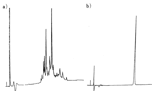
Fig. 11. HPLC of Synthetic cAP (OD at 220 nm)
