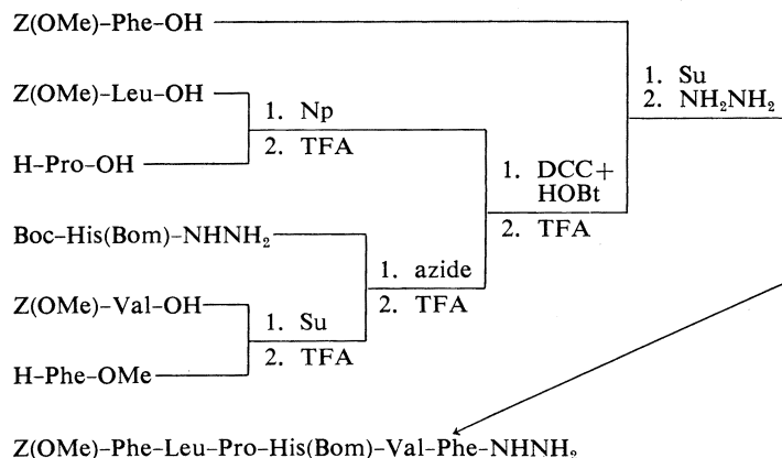
Fig. 8. Synthetic Scheme for the Protected Hexapeptide Hydrazide [7] (Positions 1—6)
