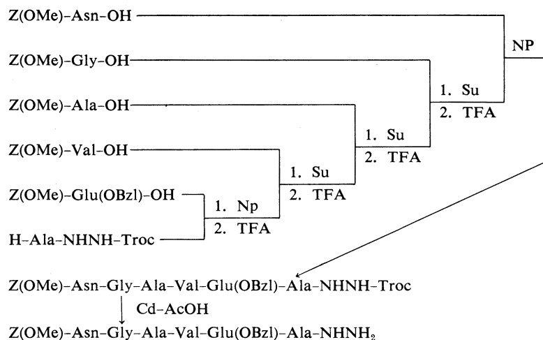
Fig. 4. Synthetic Scheme for the Protected Hexapeptide Hydrazide [3] (Positions 19–24)
