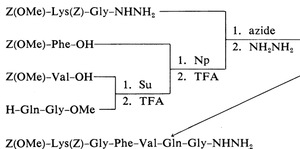
Fig. 4. Synthetic Scheme for the Protected Hexapeptide Hydrazide [3] (Positions 19–24)
