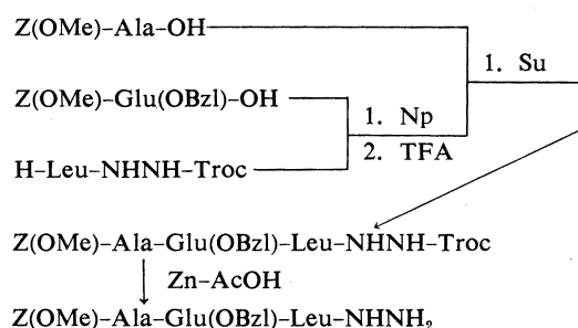
Fig. 7. Synthetic Scheme for the Protected Tripeptide Hydrazide [6] (Positions 7—9)
