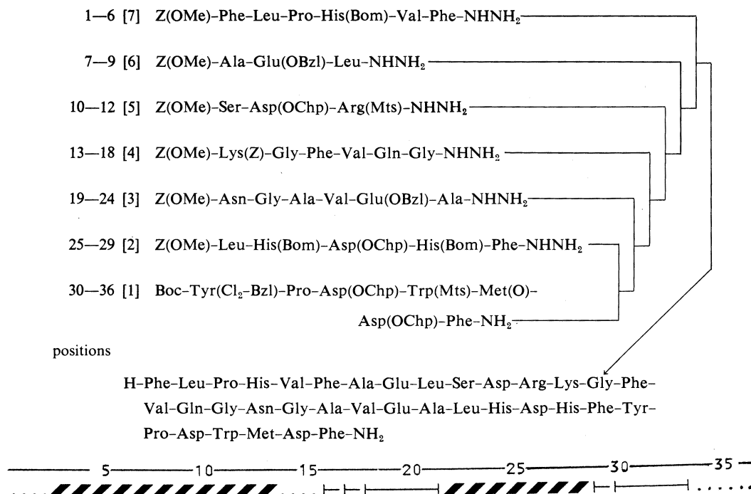
Fig. 1. Amino Acid Sequence of Chicken Antral Peptide and Chou-Fasman Prediction of Its Conformation
