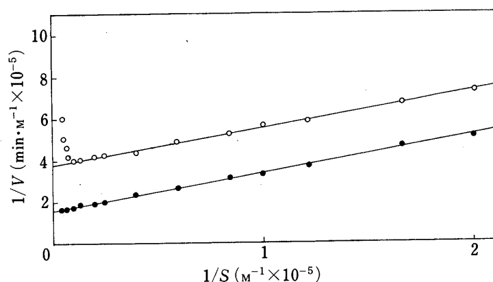
Fig. 2. Double-Reciprocal Plots for the Hydrolysis of GPA- \beta NA (O) and Arg- \beta NA (●) Catalyzed by BL-APase at 37°C in Phosphate Buffer (0.057 M, pH 7.0)
