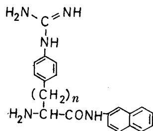
Fig. 1. Chemical Structures of GPA-βNA and GPG-βNA
