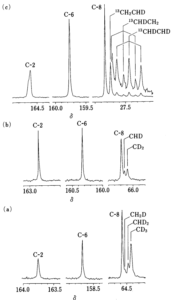
Fig. 1. Signals from p.n.d. ^{13}\text{C} -NMR Spectra of (a) 2 , (b) 4 and (c) 3 Derived from [1\text{-}^{13}\text{C}, 2\text{-}^2\text{H}_3]\text{Acetate}
