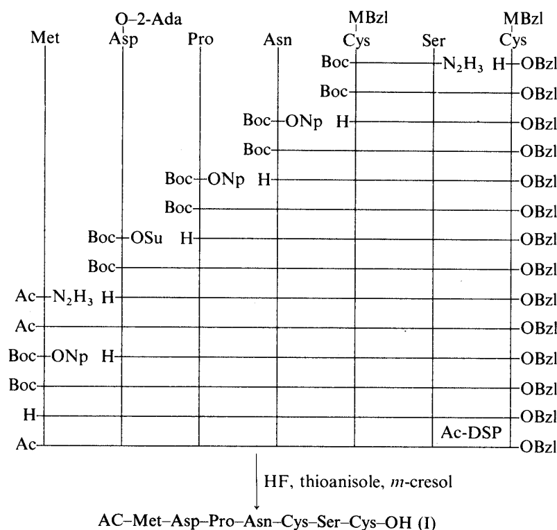
Fig. 1. Synthetic Scheme for the N-Terminal Heptapeptide Ac-(MT II 1-7)-OH of Mammalian MTs
