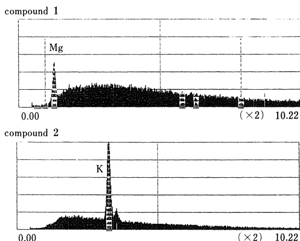
Fig. 2. Energy-Dispersive X-Ray Analyses of Compounds 1 and 2
