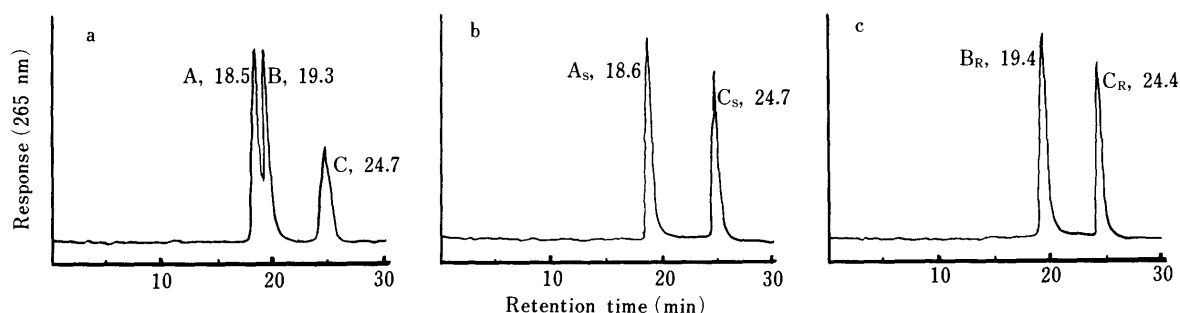
Fig. 1. HPLC Chromatograms of Oxazolam Dissolved in the Eluent
