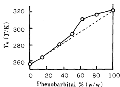
Fig. 8. Variation of T_g of the Antipyrine-Phenobarbital Binary System ----, theoretical relationship; —, observed relationship.
