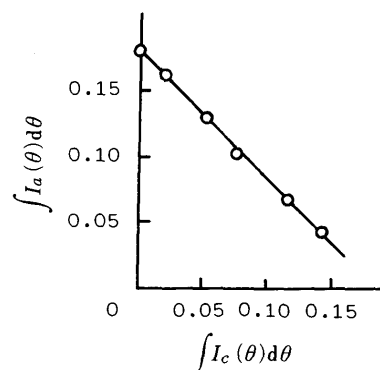
Fig. 3. The Regression Line for the Scattering Intensities from Crystalline and Amorphous Regions of Phenobarbital, Samples with Different Crystallinities Obtained by Hermans' Method
