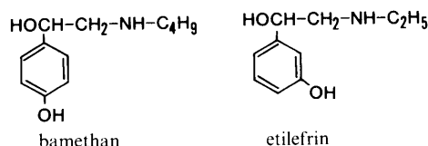
Fig. 1. Structures of Bamethan and Etilefrin
