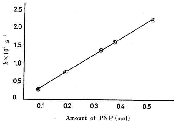
Fig. 2. Plot of Pyrolysis Rates of IIa vs. Amount of p -Nitrophenol (PNP)
