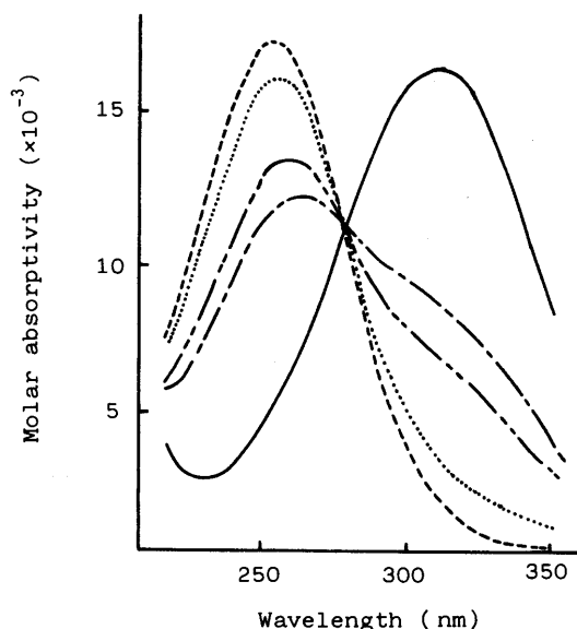
Fig. 7. UV Spectra of 5 in 20% Aqueous Dioxane at 25 °C in the Presence of 0.01 M NaHCO_3 (—); in the Presence of AcOH and AcONa (1 : 8) (---); in the Presence of AcOH and AcONa (1 : 5) (----); in the Presence of AcOH and AcONa (1 : 1) (·····) and in the Presence of 0.01 M HCl (-·-·-·-). Ionic strength 0.1.
