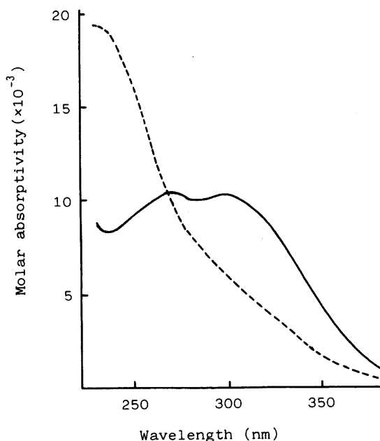
Fig. 3. UV Spectra of 2c and N -Acetyl-2,4-dinitroaniline in 20% Aqueous Dioxane in the Presence of 0.1 M HCl at 25 °C -----, 2c ; —, N -acetyl-2,4-dinitroaniline.
