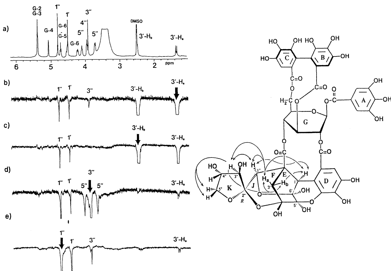
Fig. 1. 1 H-NMR (Normal and NOE Difference) Spectra of Putranjivain A (1) in DMSO- d 6
