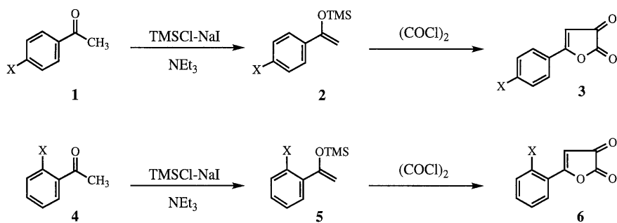
For Compounds 1 - 6
