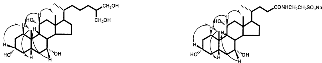
Fig. 1. Results of Two Dimensional Correlations and NOE Experiments on 3 and 5
