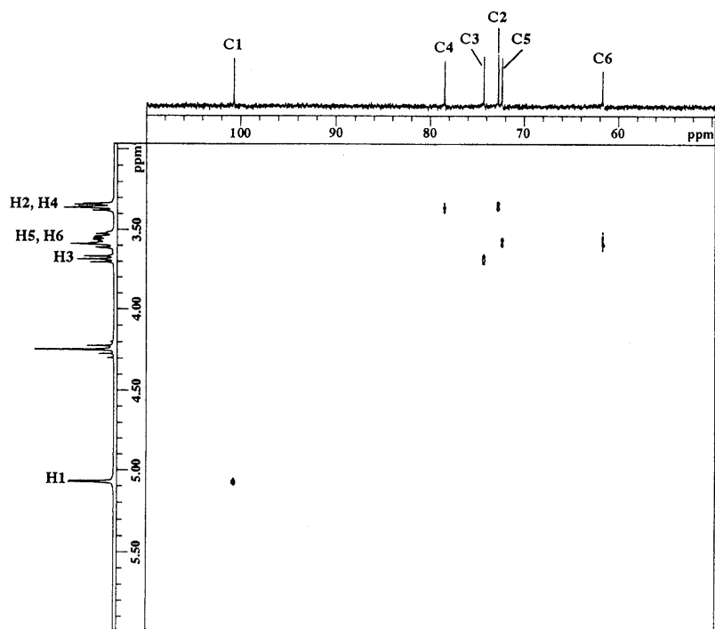
Fig. 3. ^1\text{H} - ^{13}\text{C} COSY NMR Spectrum of o -CD
