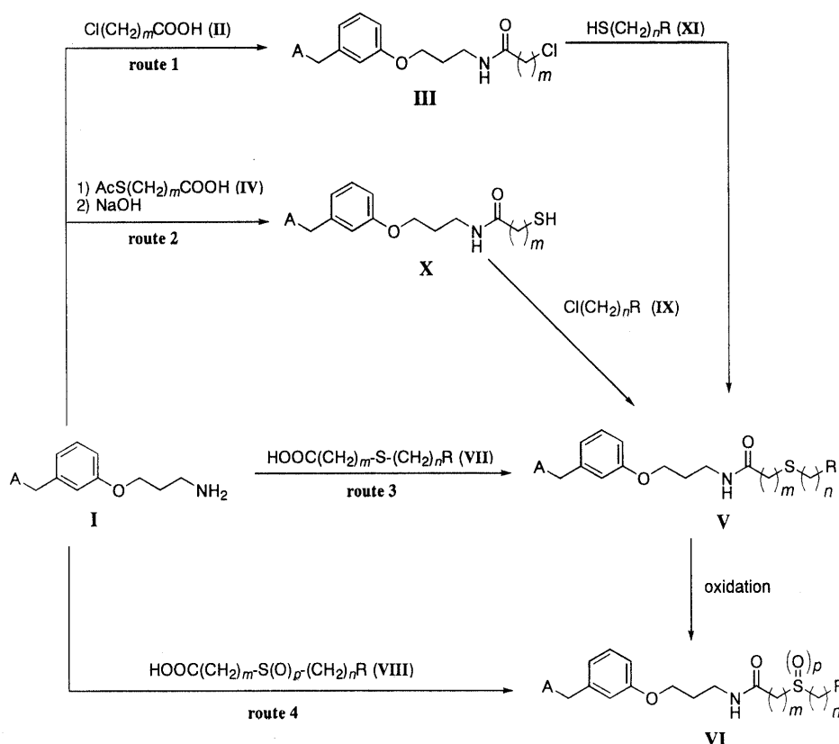
Chart 1. Synthetic Routes to N -Phenoxypropylacetamide Derivatives
