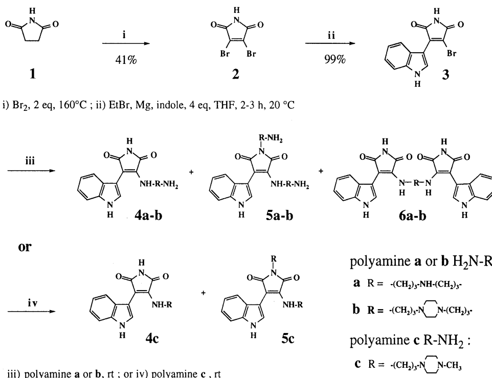
Chart 1. Synthesis of Polyamine Linked-Monoindolylmaleimide Derivatives 4–6
