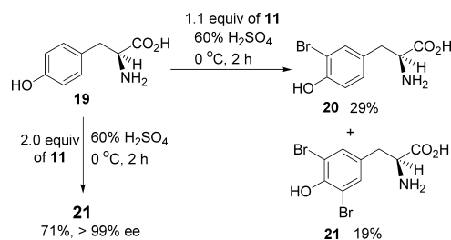
Chart 3. Bromination of L-Tyrosine ( 19 )
