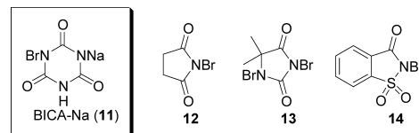
Fig. 1. Brominating Reagents
