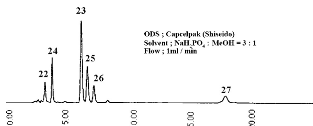
Fig. 2. HPLC Chart for the Bromination of Phenylglycine ( 22 )
