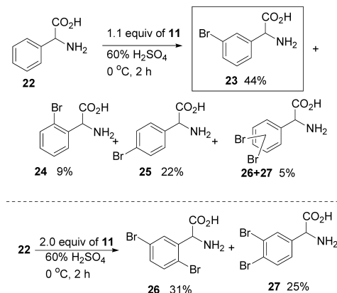
Chart 4. Bromination of dl -Phenylglycine ( 22 )
