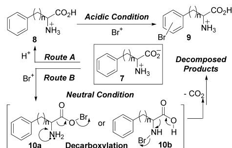
Chart 2. Direct Bromination of Aromatic Amino Acids
