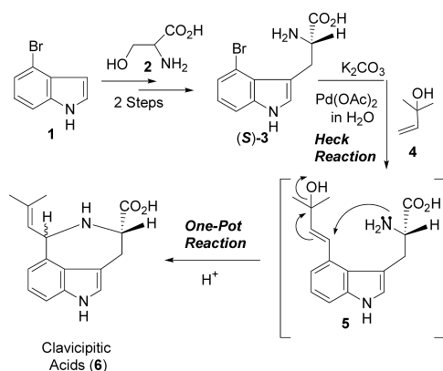
Chart 1. Three-Step Synthesis of Clavicipitic Acids ( 6 )
