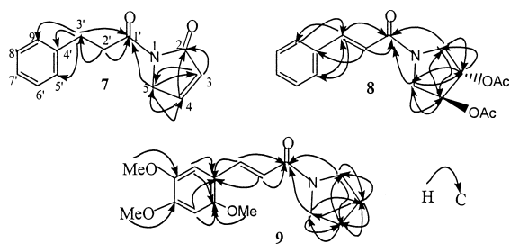
Fig. 1. 2D HMBC Correlations of 7–9
