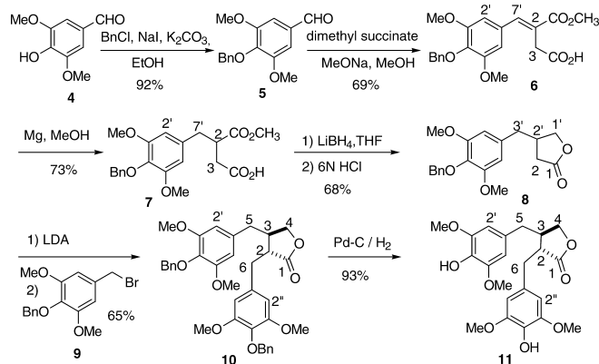
Chart 4. Synthesis of Dibenzylobutanolide 11
