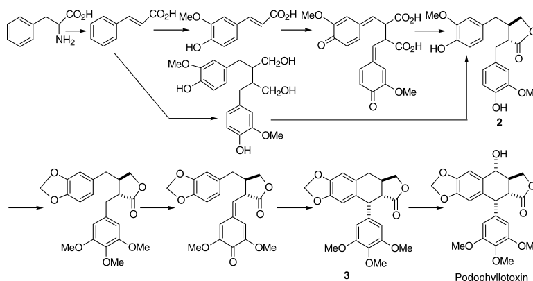
Chart 2. Proposed Biosynthetic Pathway of Podophyllotoxin
