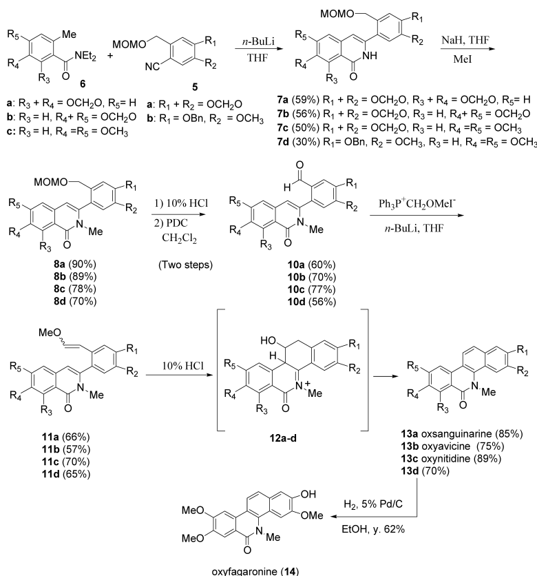
Chart 3. Synthesis of Oxyfagarone, Oxyavicine, Oxynitidine, and Oxyfagarone
