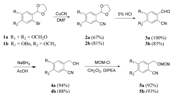
Chart 2. Synthesis of Benzonitriles 5a, b
