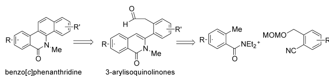
Chart 1. Retrosynthetic Pathway of Benzo[ c ]phenanthridines
