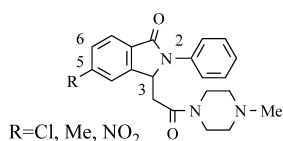
Fig. 2. Structure of 2-Phenyl-3-[2-(4-methyl-1-piperazinyl)-2-oxoethyl]-5-Chloro, Methyl and Nitroisindolin-1-one
