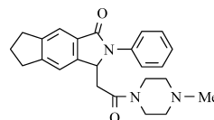
Fig. 3. Structure of 47 ( JM-1232 )
