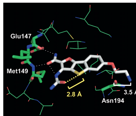
Fig. 4. The X-Ray Structure of JNK3 with 16k
