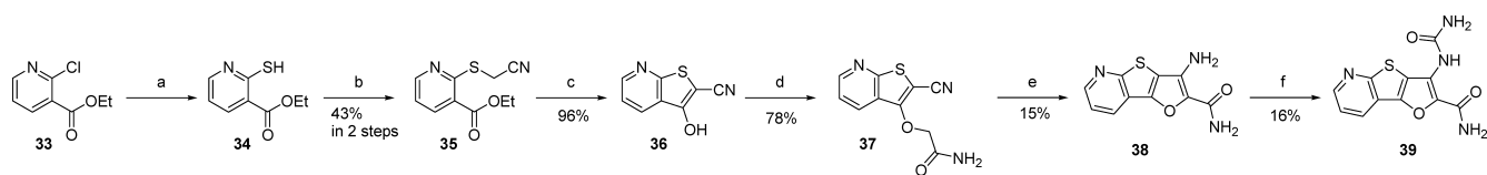
Chart 5. Synthesis of Furo[2',3':4,5]thieno[2,3- b ]pyridine Derivative
