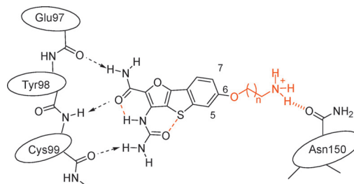
Fig. 3. Predicted Binding Model Orientated to Interact with Asn150
