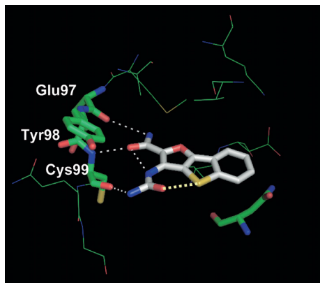
Fig. 2. Predicted Binding Mode of 13a with IKK \beta
