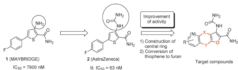
Fig. 1. Drug Design of the Tricyclic Furan Derivative
