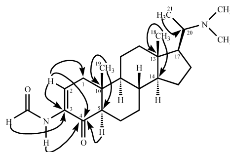
Fig. 1. Selected HMBC Correlations in Compound 1
