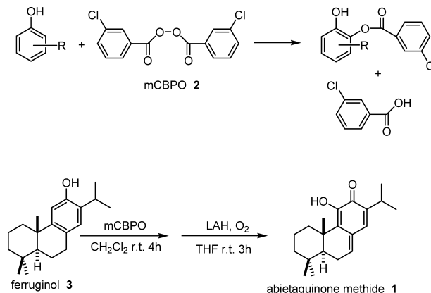
Fig. 1. ortho -Oxidation of Phenols with m CBPO
