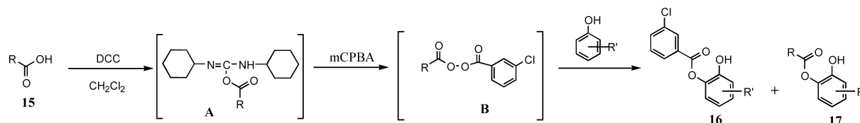
Fig. 3. Synthesis of Asymmetric Diacyl Peroxides and Oxidation of Phenols with Asymmetric Diacyl Peroxides
