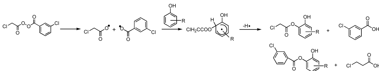
Fig. 4. Presumed Reaction Mechanism of Oxidation of Phenols with CAMCBPO
