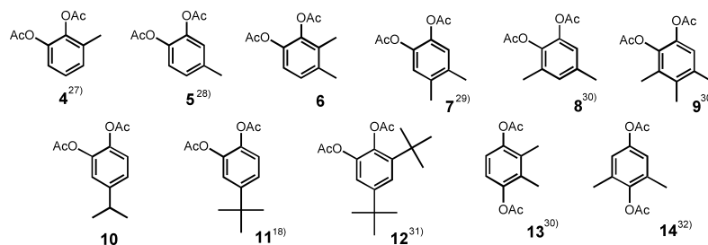
Fig. 2. Oxidation Products of Various Phenols with m CBPO and Chloroacetyl m -Chlorobenzoyl Peroxide (CAMCBPO)
