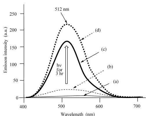
Fig. 1. Change in Emission Spectra of 5 \mu\text{M} 3 (BS-Caged- \text{L}^1 ) at pH 7.4 (10 mM HEPES with I=0.1 ( \text{NaNO}_3 )) and 25^\circ\text{C} upon Photoirradiation
