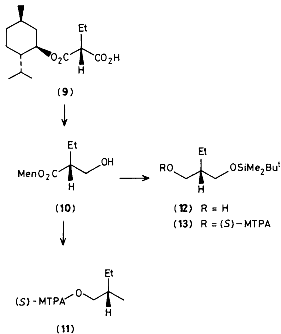
Scheme 3. Men = menthyl.
