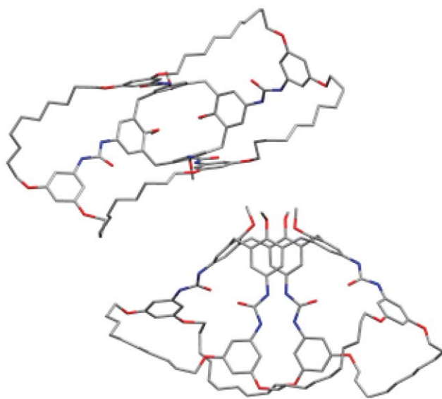
Fig. 1 Single crystal X-ray structure of the tetraloop compound 6 ( m = 10 , Y = \text{CH}_3 ); one of two crystallographically independent molecules is shown from two perspectives.
